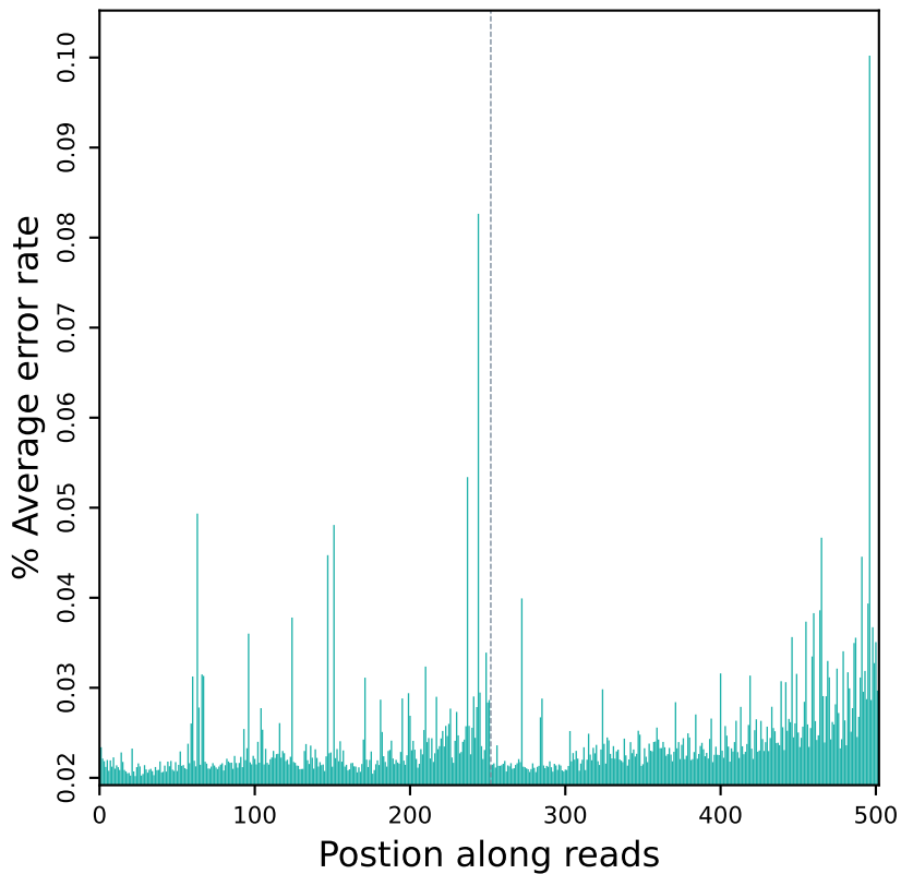
Error rate distribution along reads (R10106)
